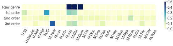
Figure 7: Attention weights of a third-order salient feature example ( Toy story 2 , 1999)
