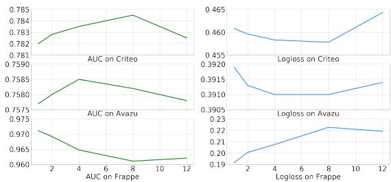
Figure 3: Sensitivity on number of heads in Transformer
